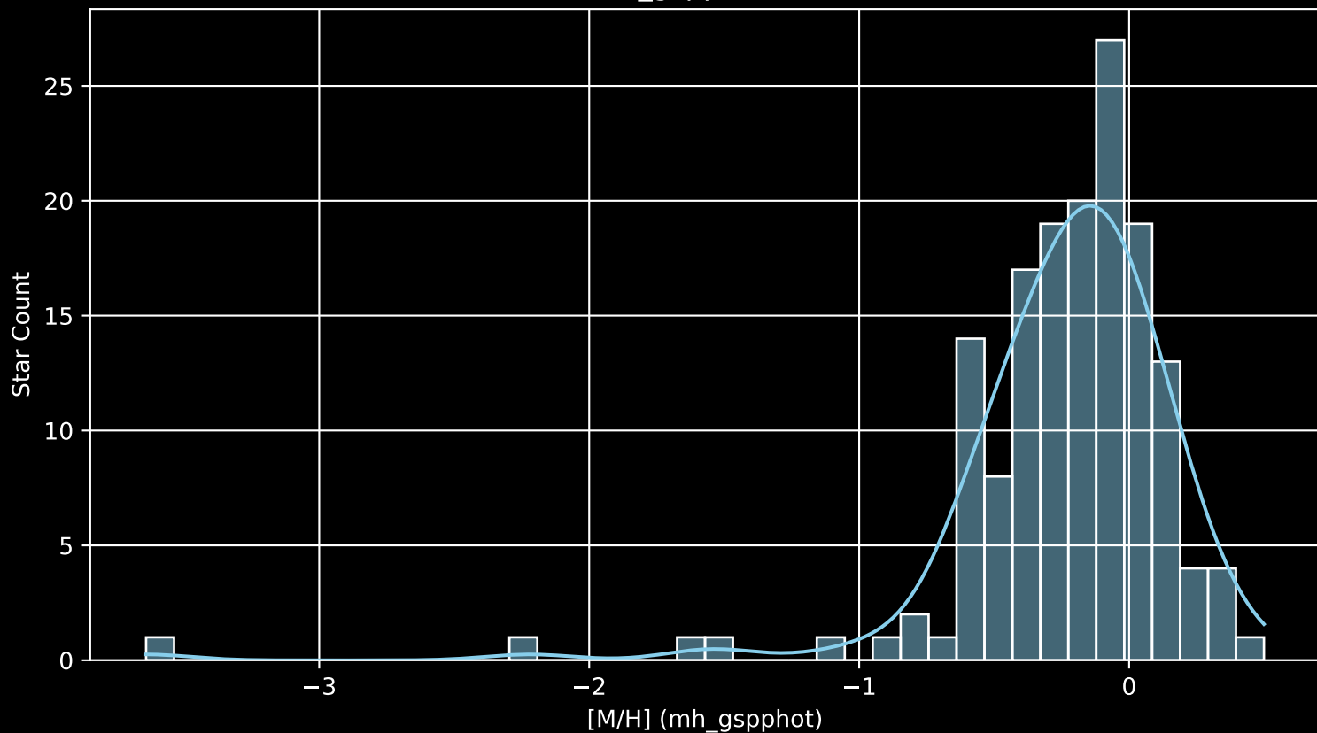
APOGEE DR17 Field: [200+25_MGA [M/H] (mh_gspphot) (n= 155)
