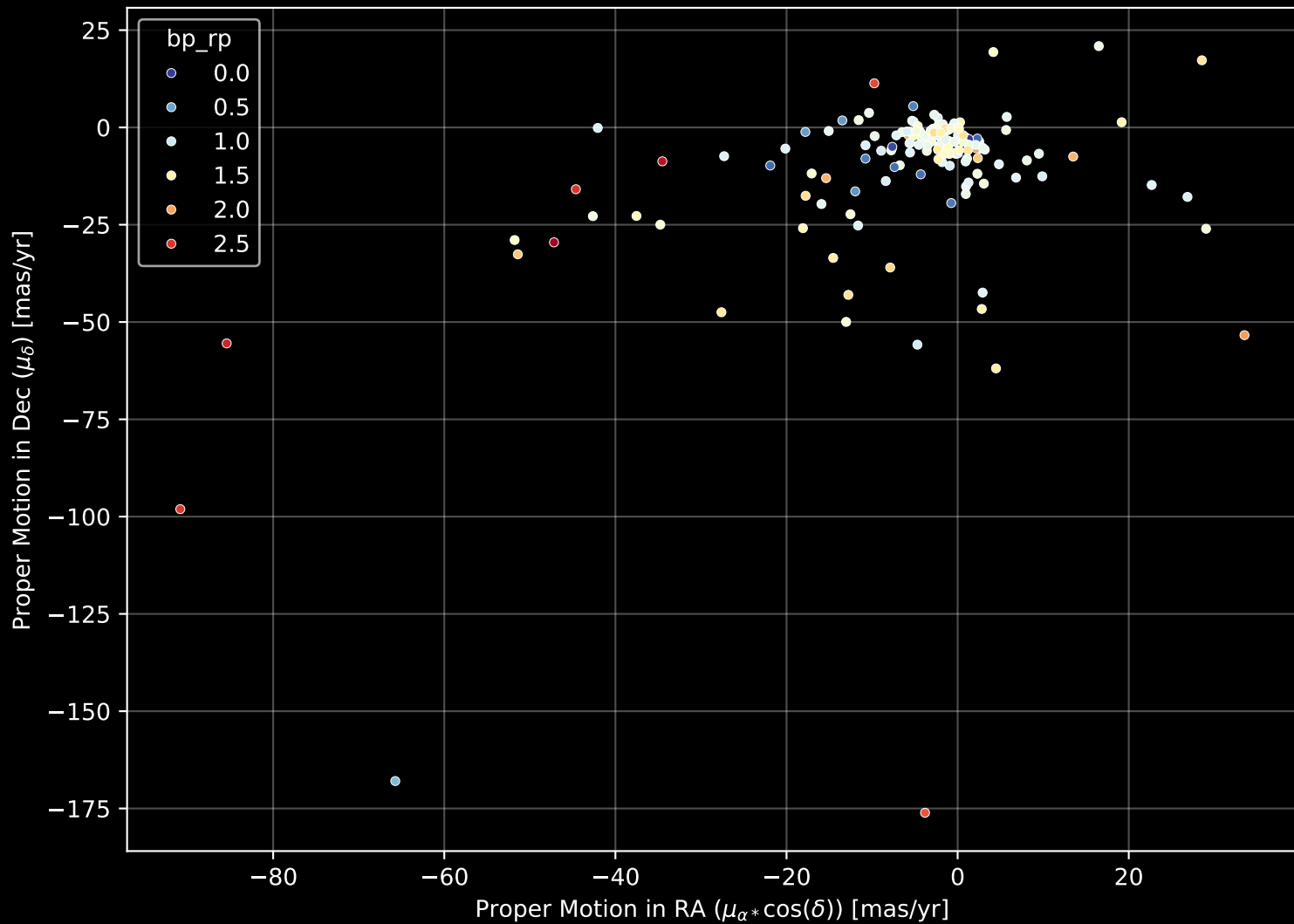
APOGEE DR17 Field: [200+25_MGA] Proper Motion Diagram (n= 162)
