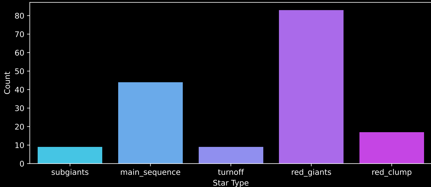
APOGEE DR17 Field: [200+25_MGA] Count plot of Star Type
