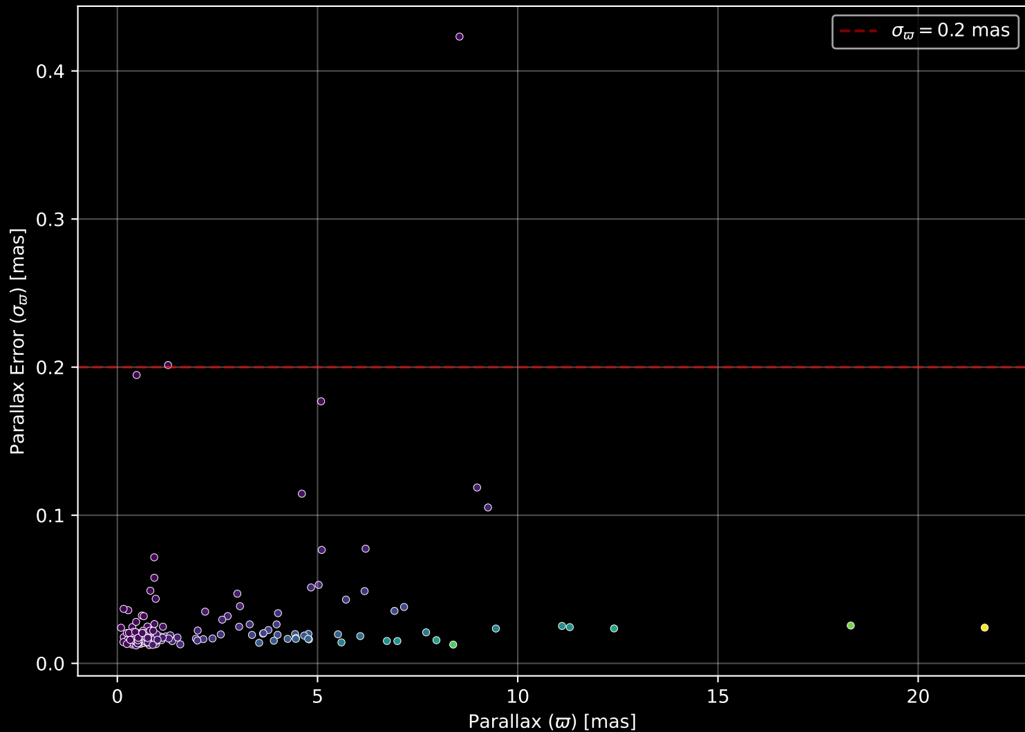
APOGEE DR17 Field: [200+25_MGA] Parallax Quality (n= 162)
