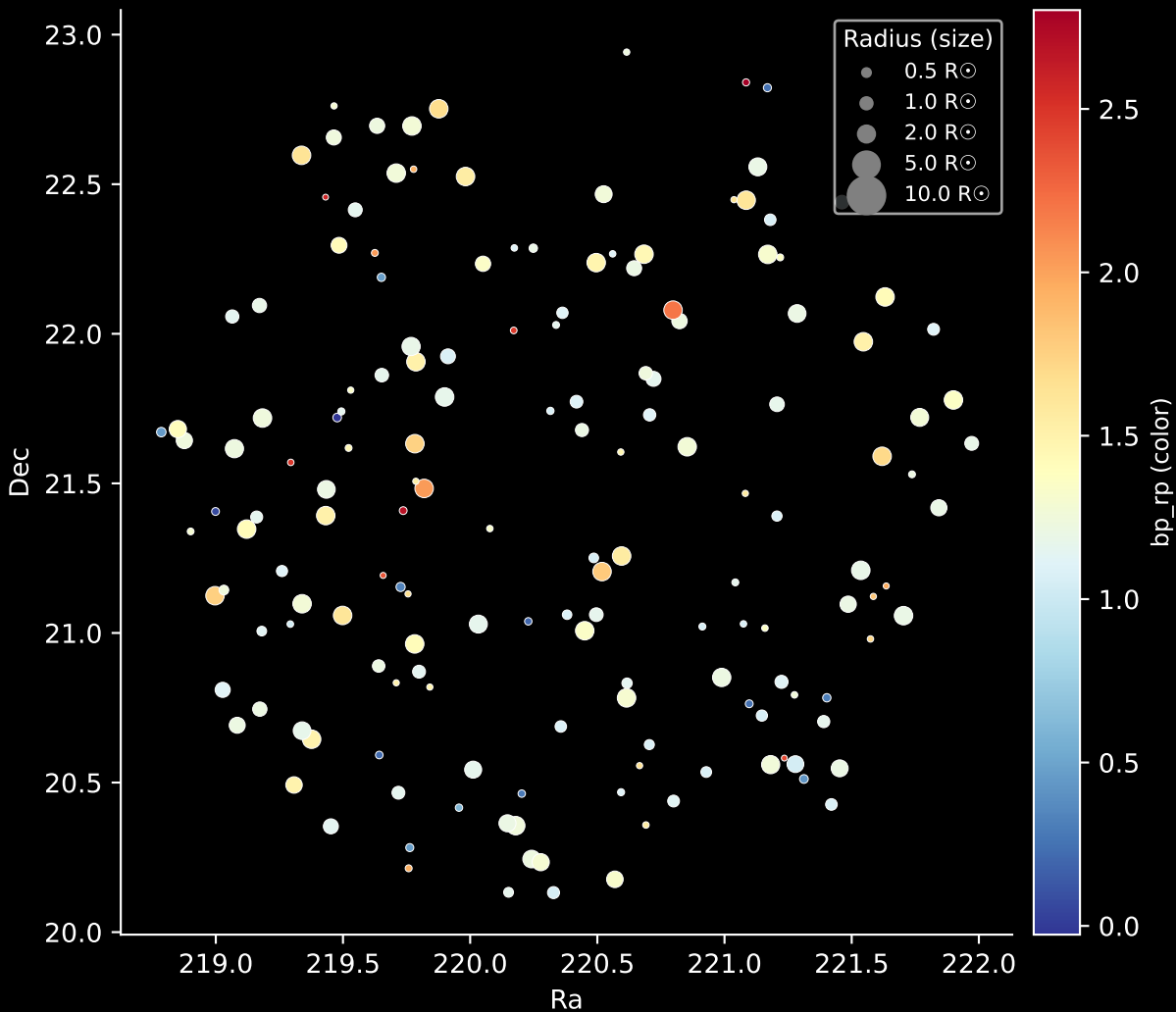
APOGEE DR17 Field: [200+25_MGA] Stars: 162
