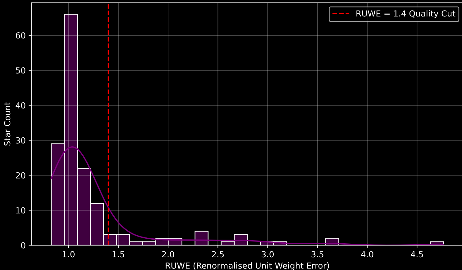
GAPOGEE DR17 Field [200+25_MGA] RUWE Distribution (n= 154)
