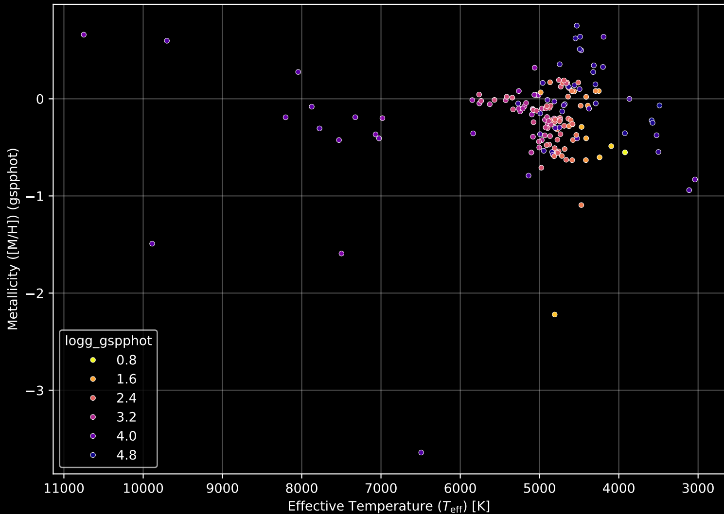
APOGEE DR17 Field: [200+25_MGA] Stellar Population Parameters (n= 162)
